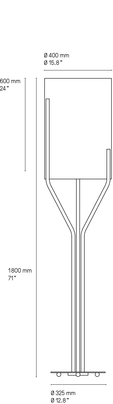
Lampadaire – Floor lamp XL
