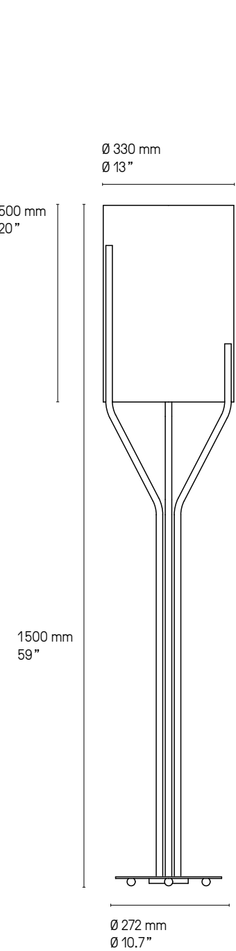
Lampadaire – Floor lamp S
