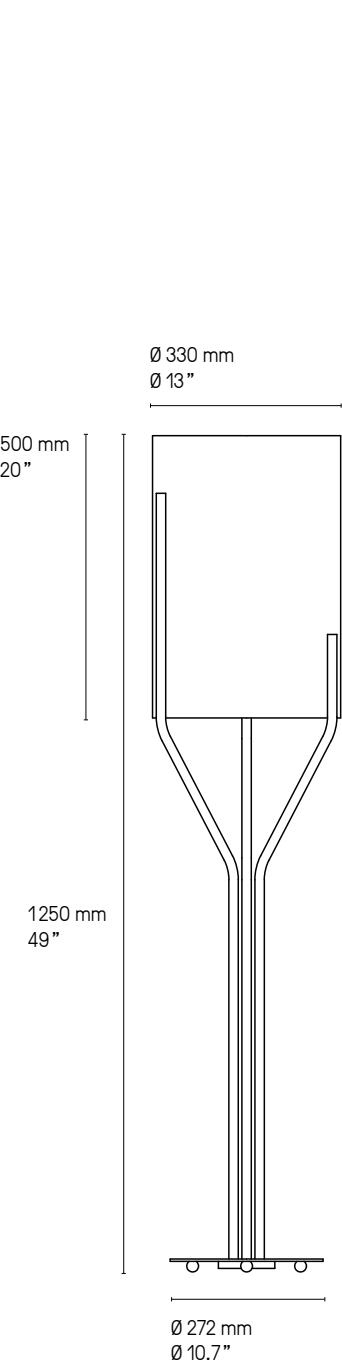
Lampadaire – Floor lamp XS
