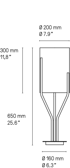
Lampe de table – Table lamp XS
