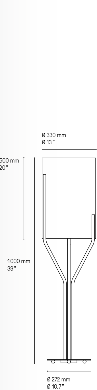
Lampadaire – Floor lamp XXS
