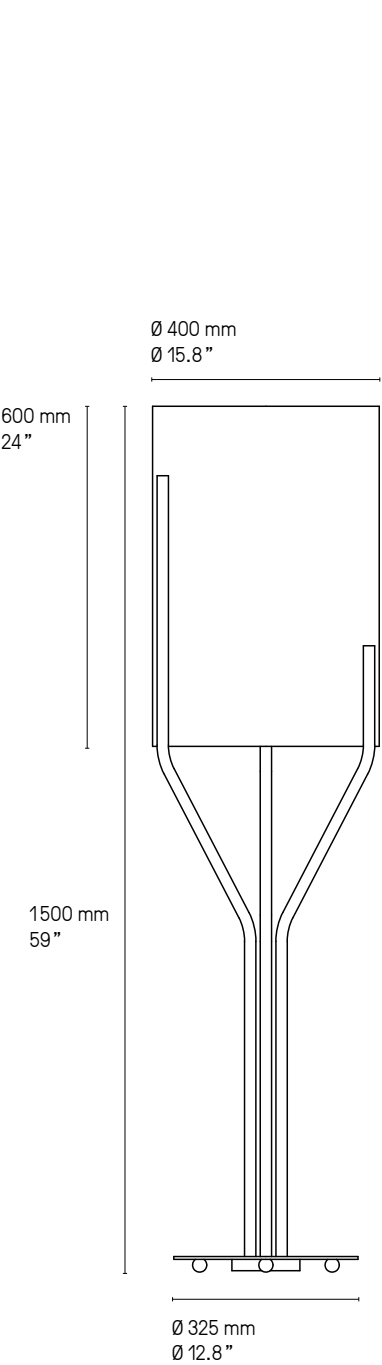
Lampadaire – Floor lamp L
